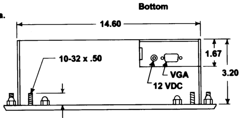
Drawing # 94-402 | 15.1 TFT LCD with machined bezel
