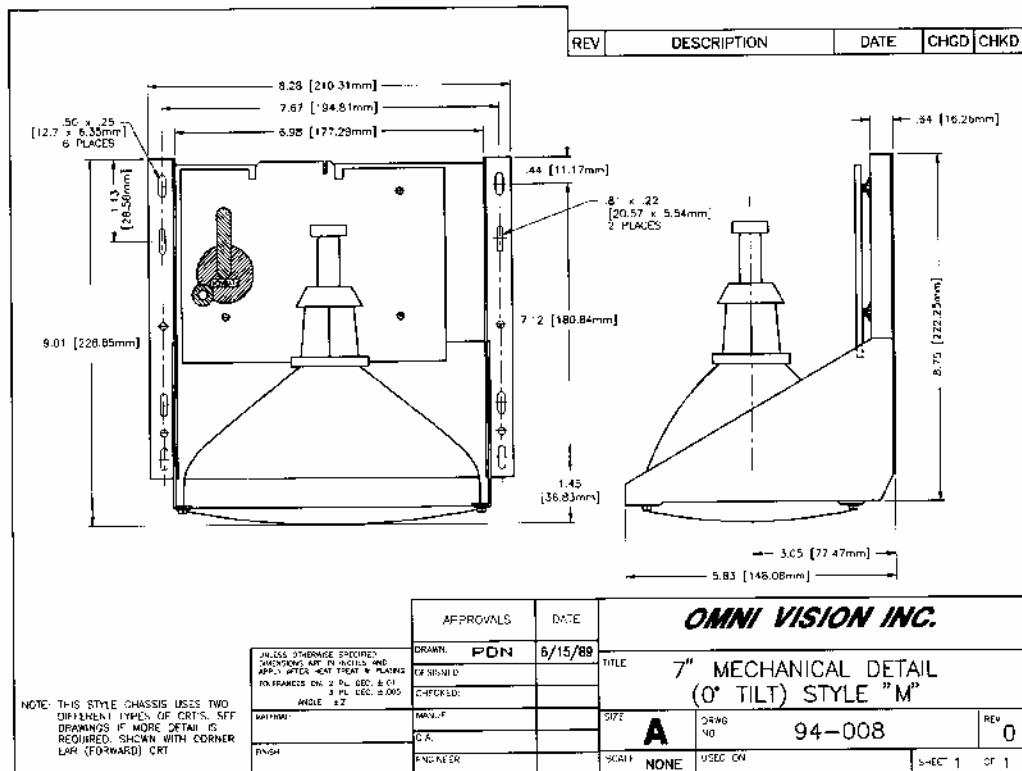
Drawing 94-008
