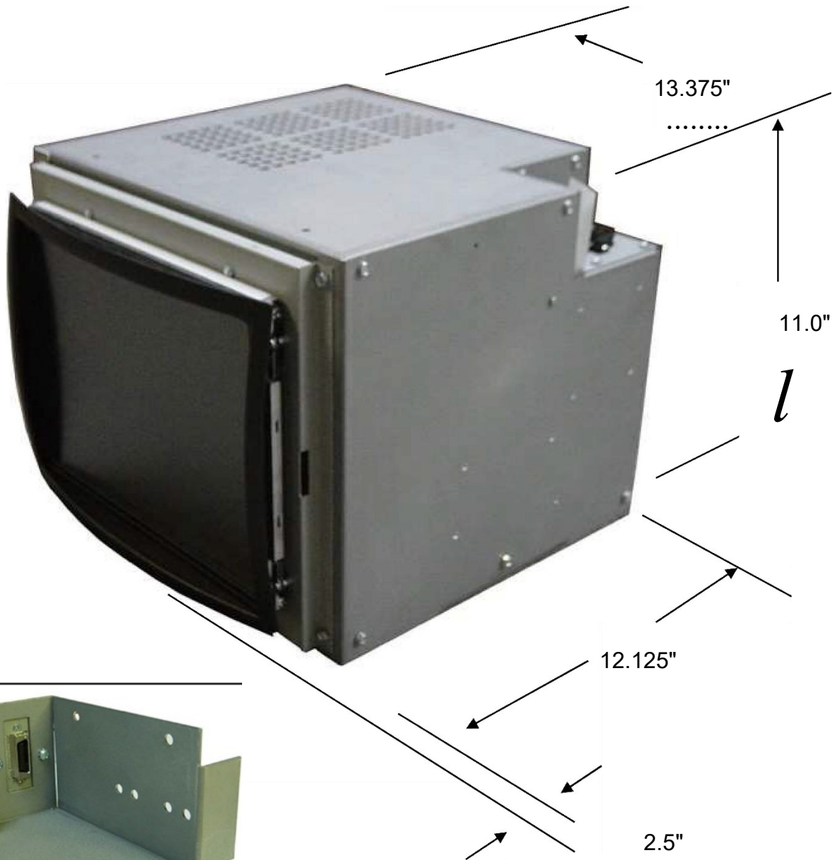
Mounted in rear: Signal and power inputConnectors
